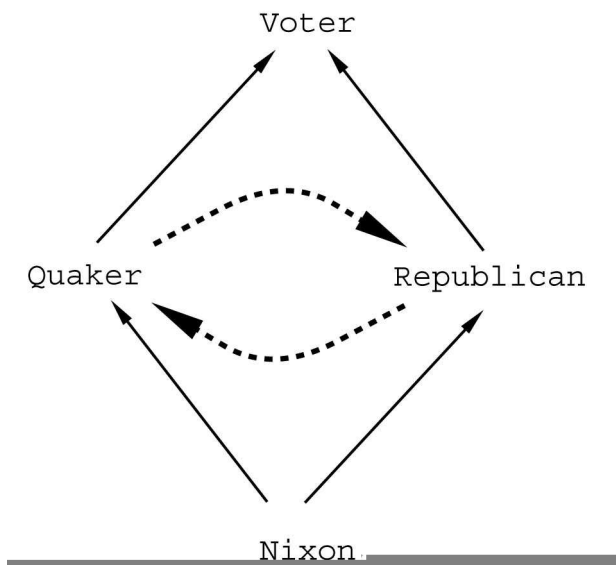
Figure 6: The extended Nixon diamond.
